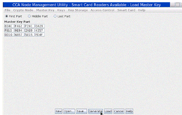
Figure 204. Load Master Key from Clear Parts — key part randomly generated
