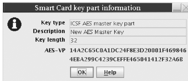
Figure 280. Secure key part entry — AES key part information for a master key
