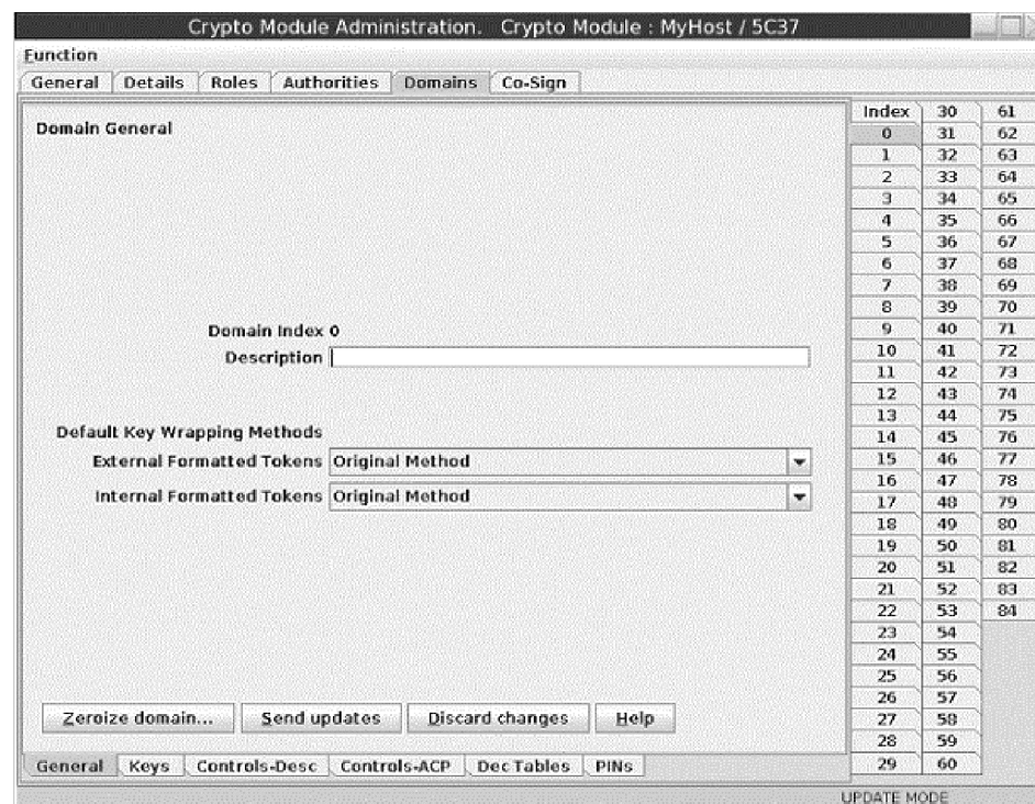
Figure 77. Domain General page
