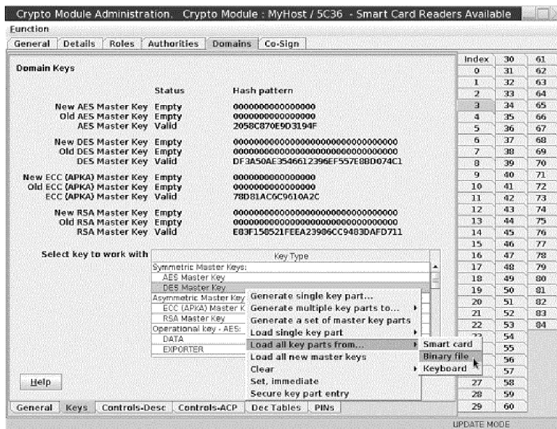
Figure 95. Load all key parts from
