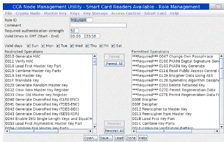
Figure 190. Role Management window modifying role attributes
