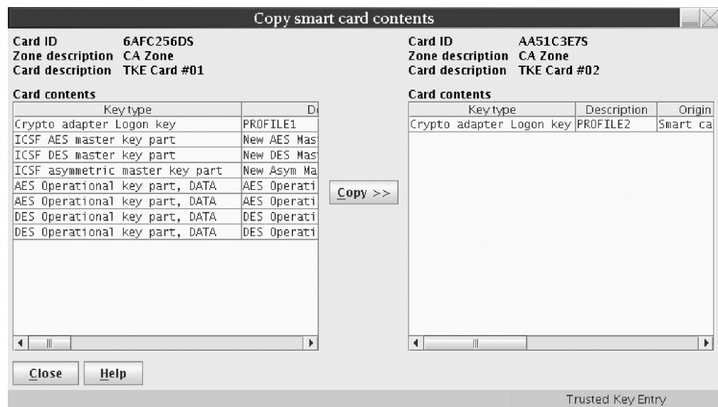
Figure 63. Select keys to copy
