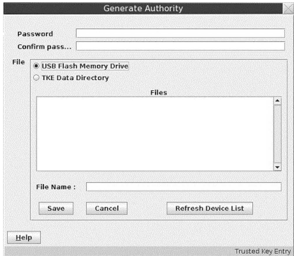
Figure 69. Save authority signature key
