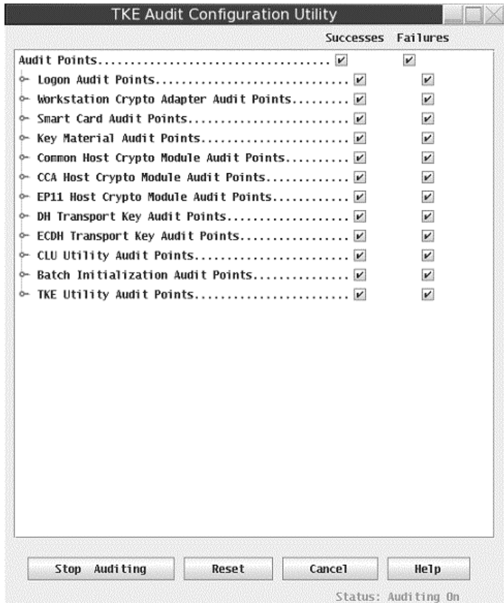
Figure 158. Default settings for auditing
