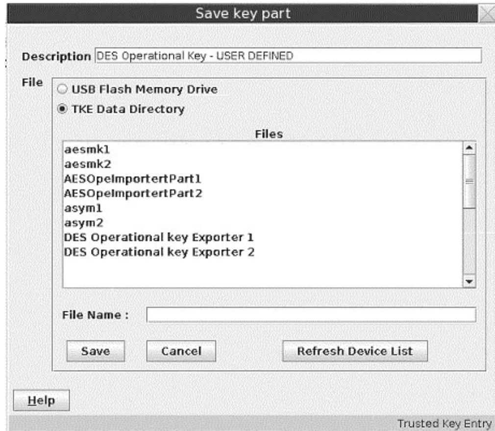
Figure 107. Save key part
