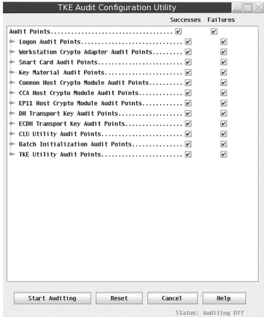
Figure 159. Auditing is off
